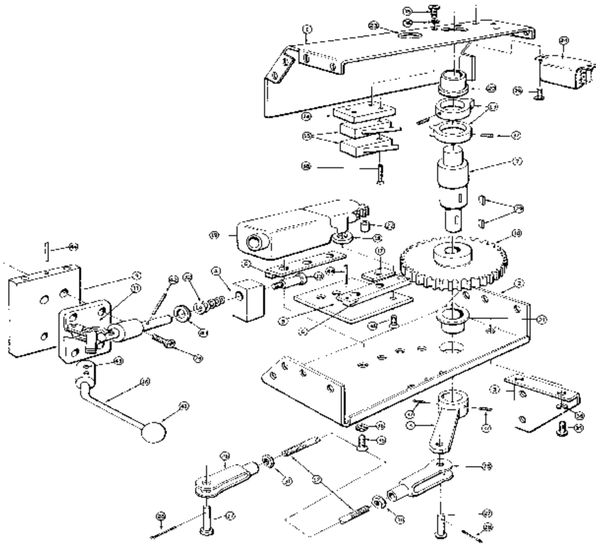
FIGURE 2 — Excell School-Bus Door Control Model 8901-001
