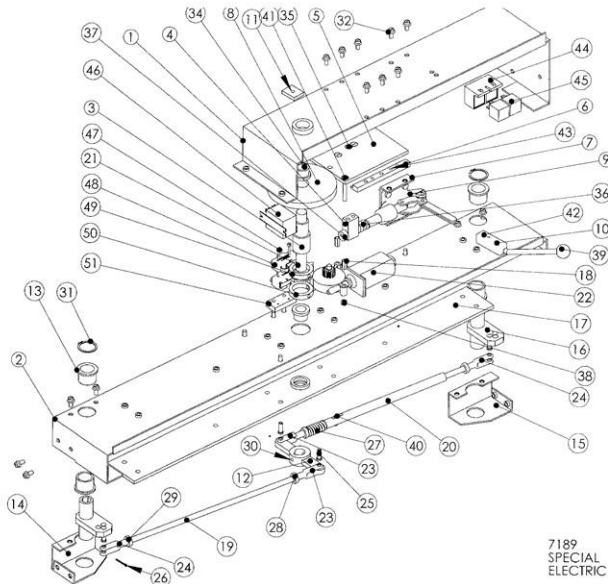
Model 7189-001 - Parts list
